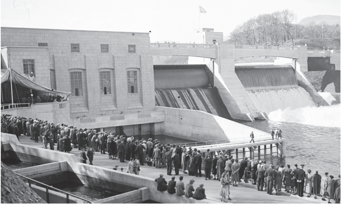
5.7 Opening ceremony at Pitlochry Power Station, 1951, Tummel valley hydroelectric scheme. © The Scotsman Publication Ltd. Licensor www.scran.ac.uk
