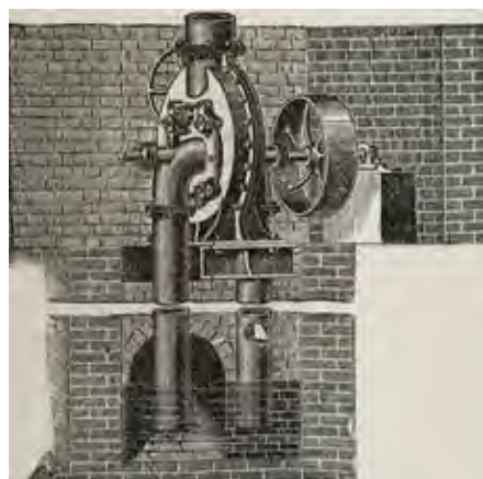
Vortex Turbine at Marsh Mills, Plympton
